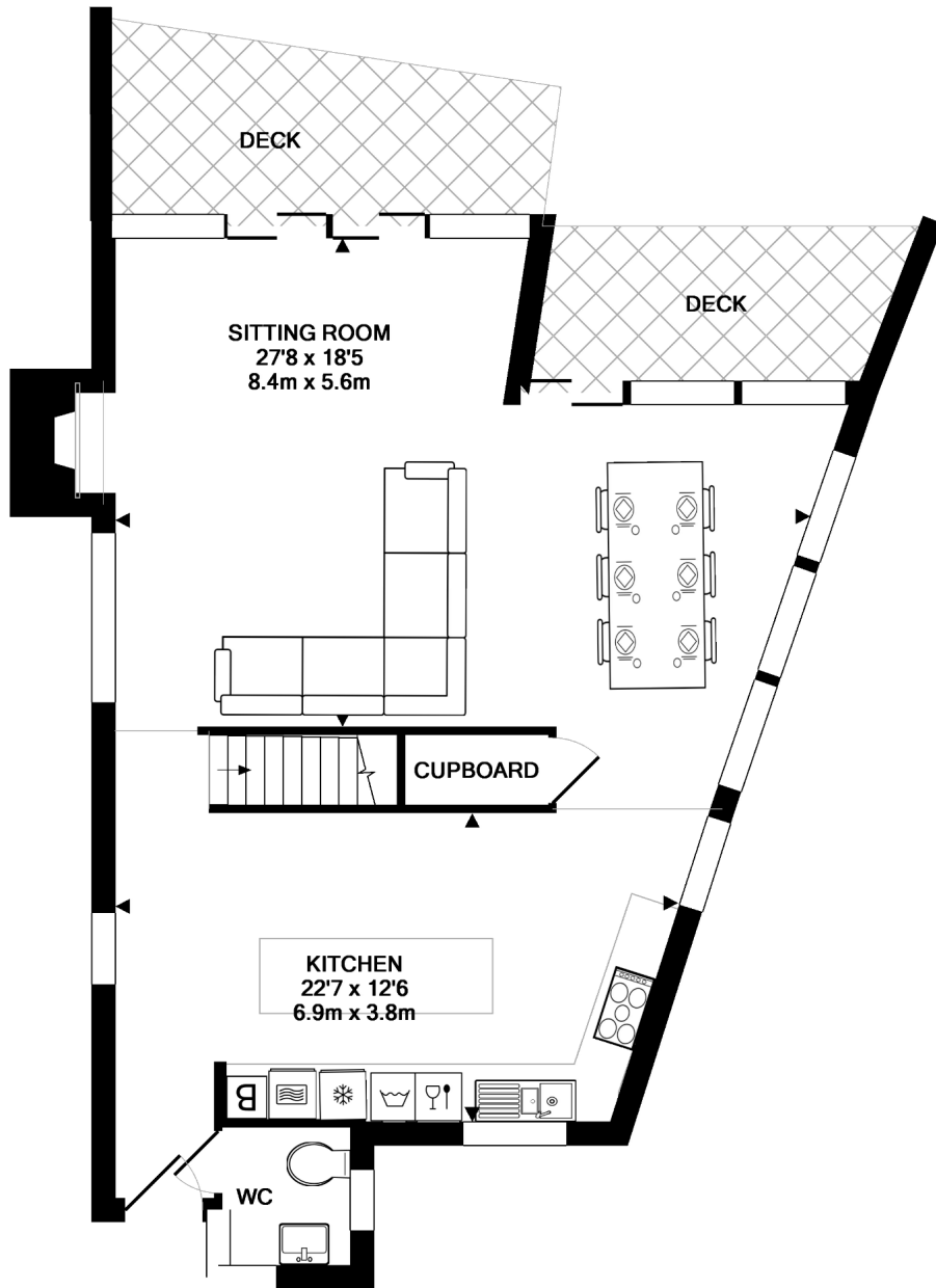
GROUND FLOOR APPROX. FLOOR AREA 867 SQ.FT. (80.6 SQ.M.)
