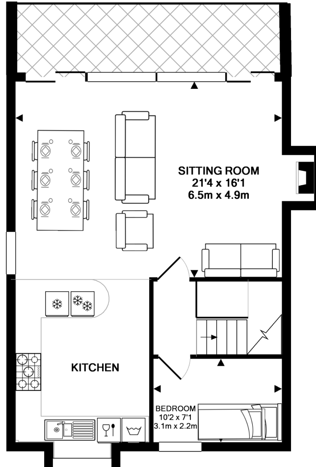
1ST FLOOR APPROX. FLOOR AREA 626 SQ.FT. (58.1 SQ.M.)
